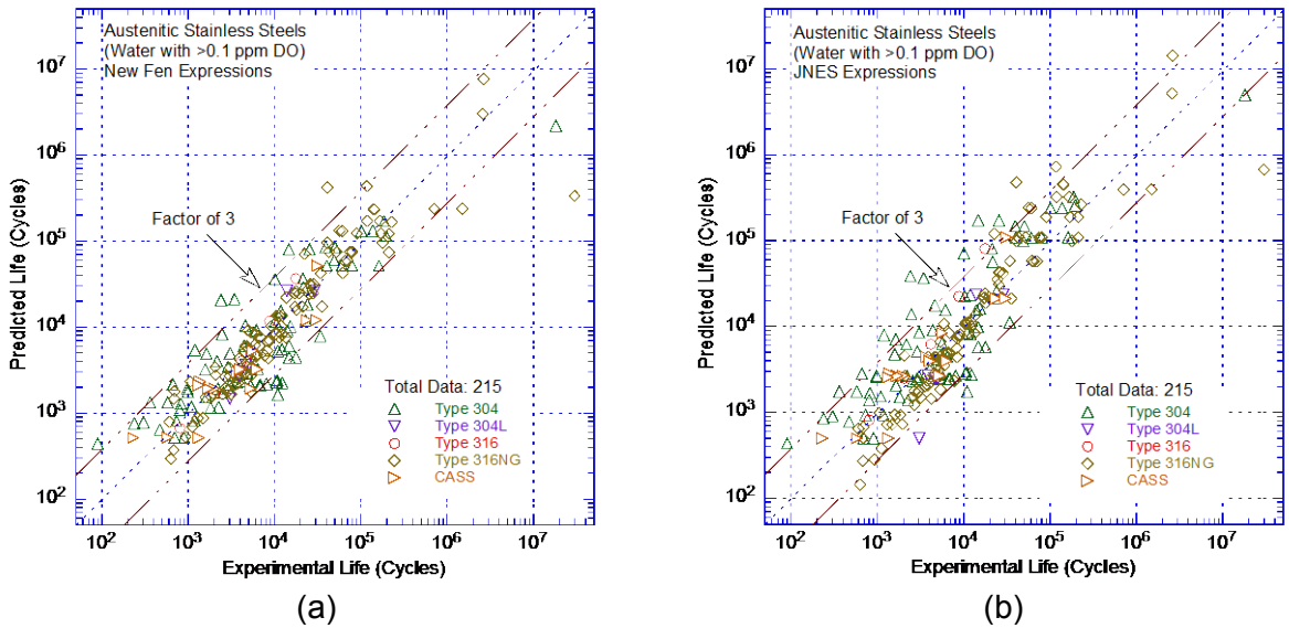
Figure 105. Experimental fatigue lives of wrought and cast austenitic SSs in water containing greater than 0.1 ppm DO vs. fatigue lives predicted from (a) the updated ANL expression and (b) the JNES expression.
