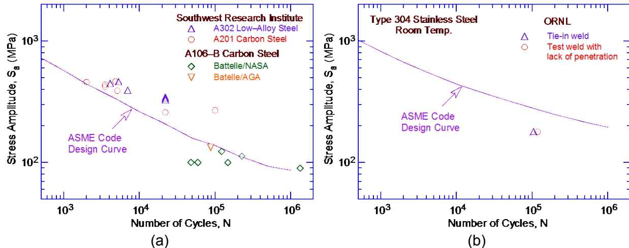
Figure 120. Fatigue data for (a) carbon and low-alloy steel and (b) Type 304 stainless steel components (Refs. 237,238).
